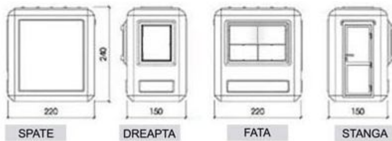
CABINA PAZA 2200X1500X2400 mm
